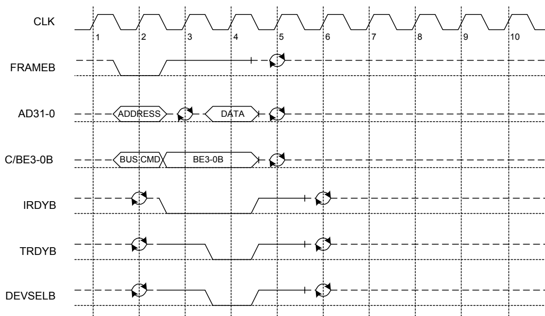
Figure 12. I/O Read
