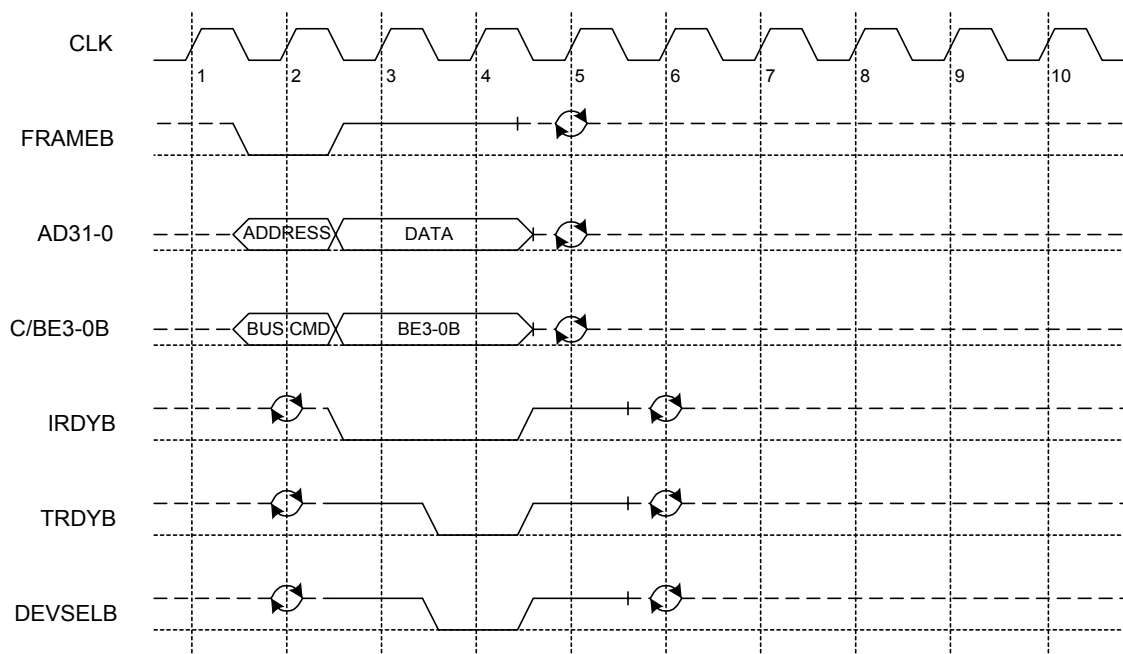
Figure 13. I/O Write
