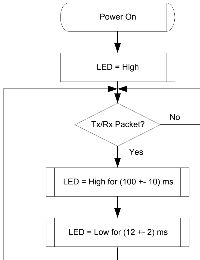
Figure 5. TX/RX LED
