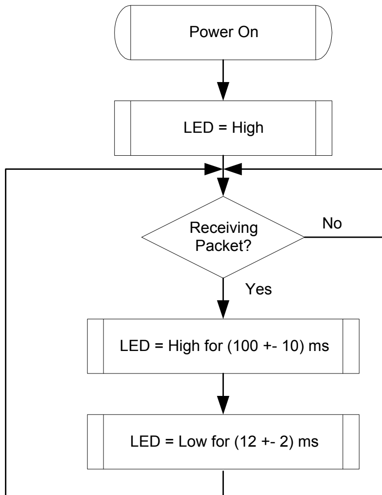
Figure 3. RX LED
