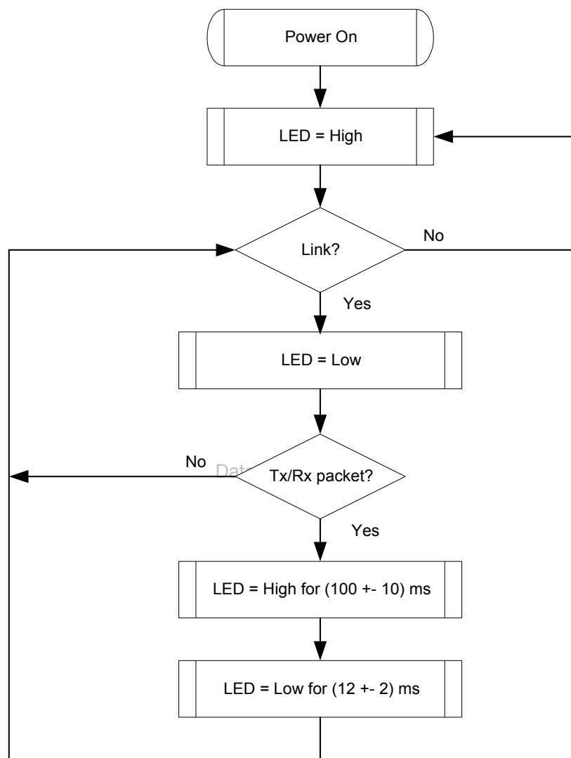
Figure 6. LINK/ACT LED
